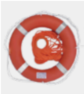
CSS Test Lifebuoy Specifications: Diameter 71 cm, Inner diameter 44 cm Model: Marine Lifebuoy (CSS Type)
